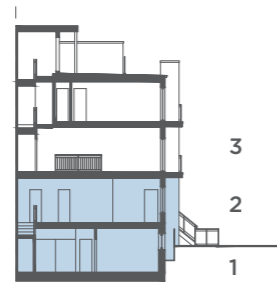
BLOCK 1 & 2 - TYP. SECTION
